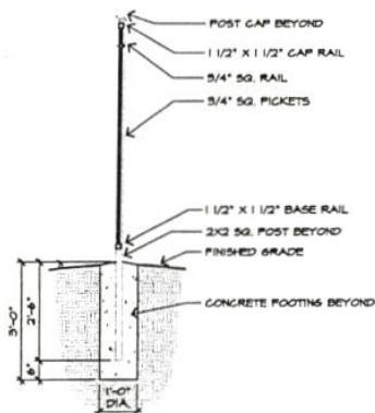
2 ORNAMENTAL STEEL FENCE SECTION
