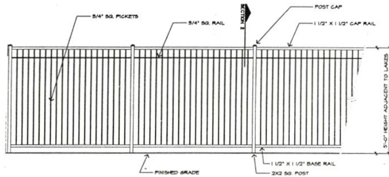
1 ORNAMENTAL STEEL FENCE ELEVATION
